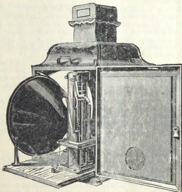
HEADLIGHT LAMP.
