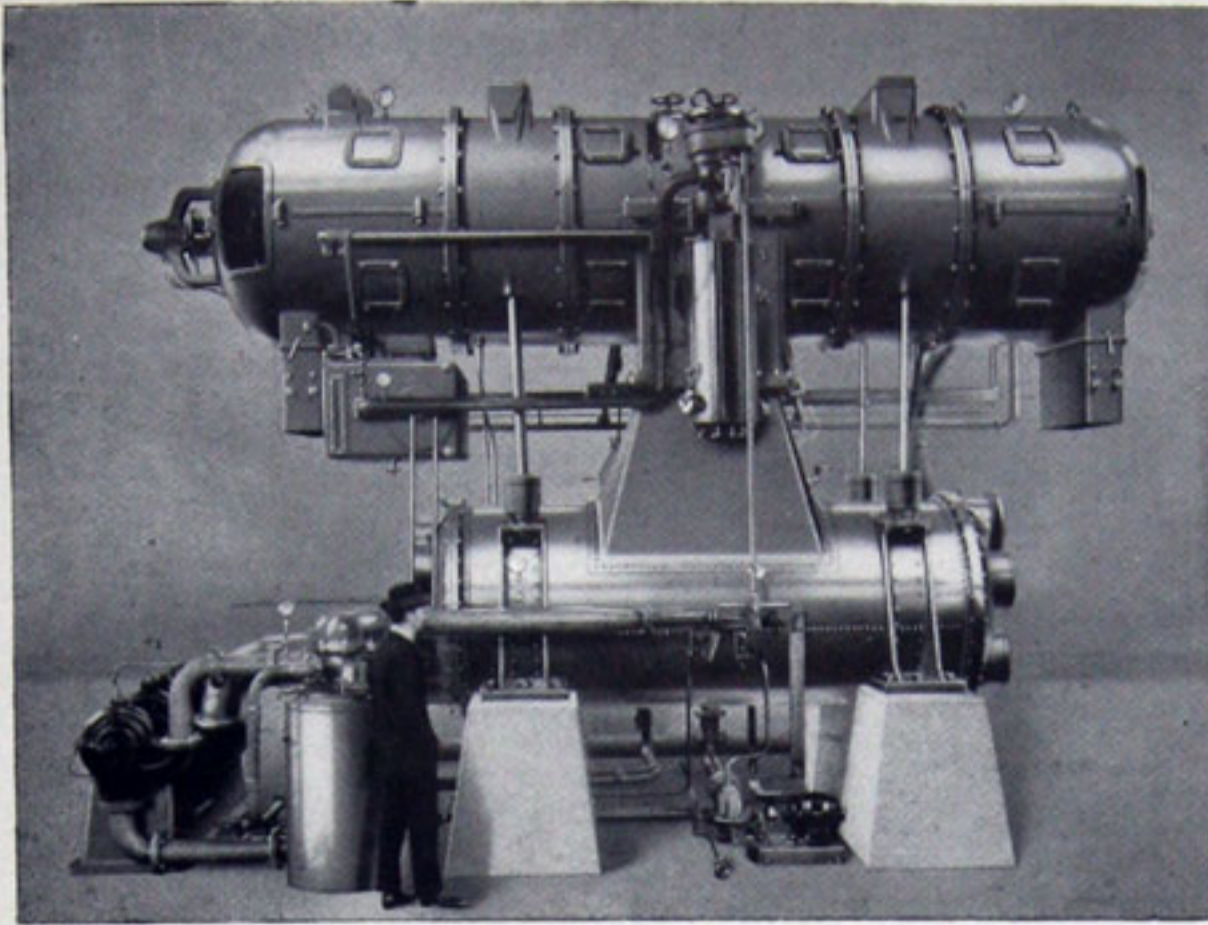
BRUSH-LJUNGSTROM TURBO-GENERATOR
