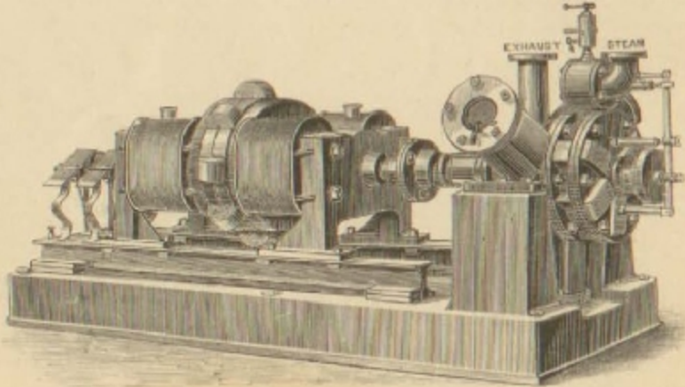
BRUSH DYNAMO CONNECTED DIRECT TO BROTHERHOOD ENGINE.
